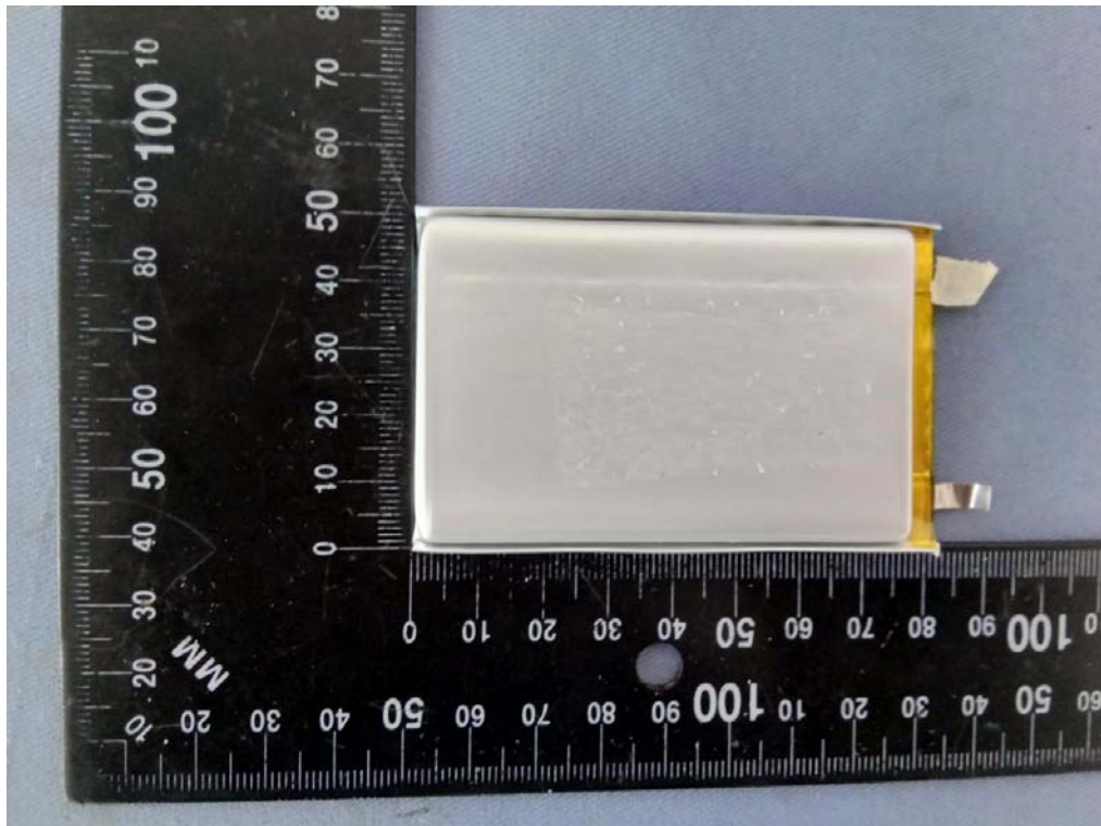
Figure 3 Overall view I of cell (电芯图 I)
